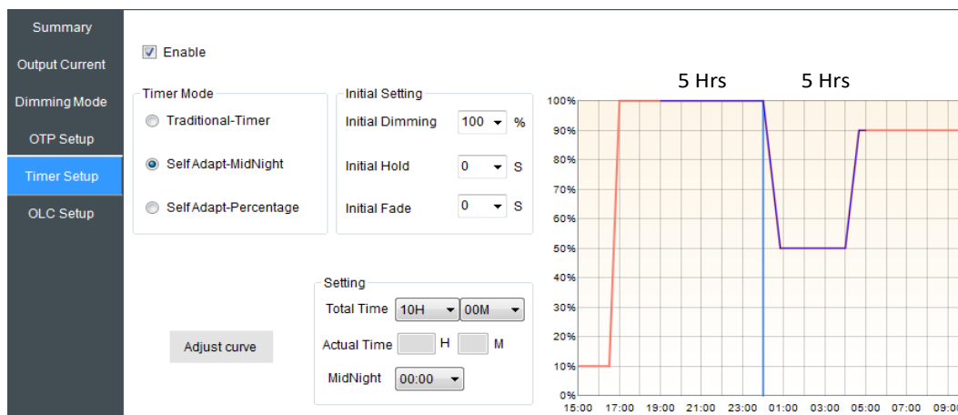
Figure 28: Self Adapt-MidNight 10 Hours ON
