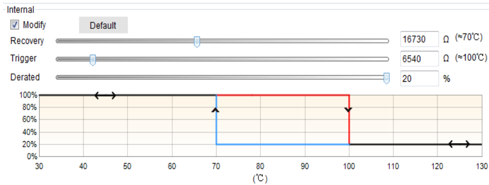
Figure 36: Internal OTP Setting
