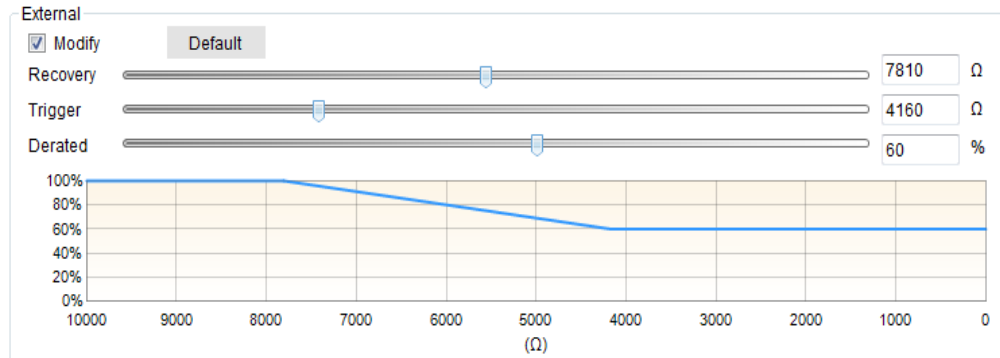
Figure 35: External OTP Setting
