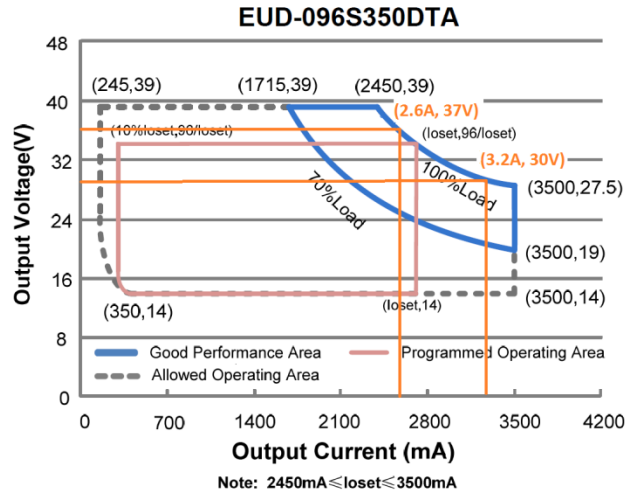
Figure 7: Upper Voltage Limit Varies Depending on loset
