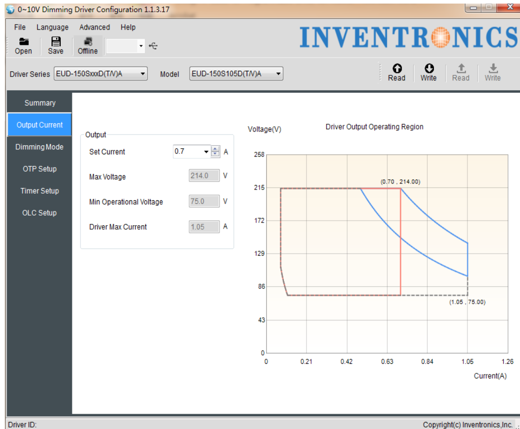
Figure 15: 0-10V Dimming Driver Configuration Window
