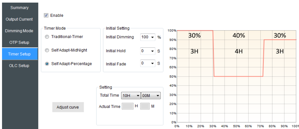
Figure 30: Self Adapt-Percentage 10 Hours ON
