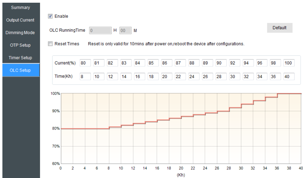
Figure 32: Output Lumen Compensation Setting
