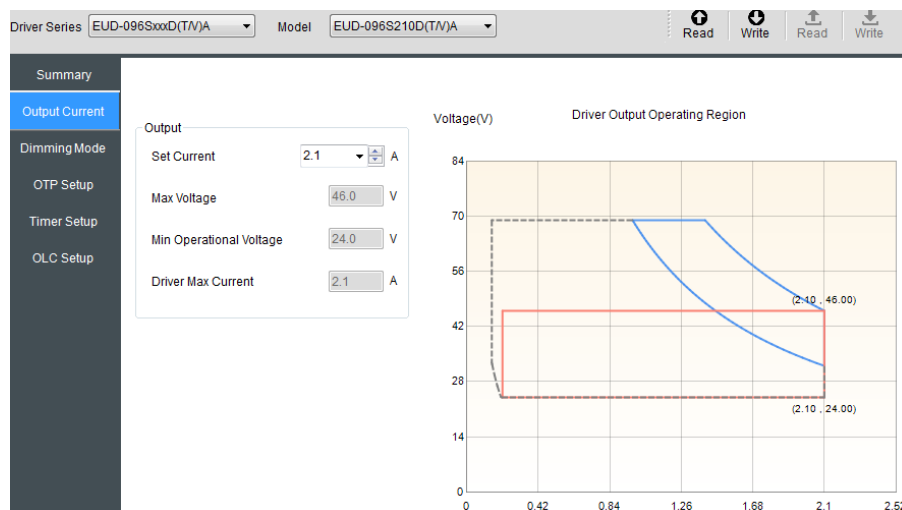
Figure 18: Software Interface Default Current Setting
